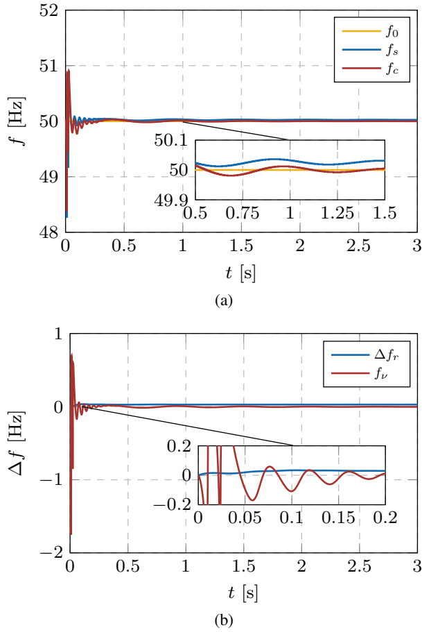
Fig. 4: Frequency response of the virtual machine emulator during start-up: (a) Initial and computed frequency terms. (b) Contribution of different frequency components.
