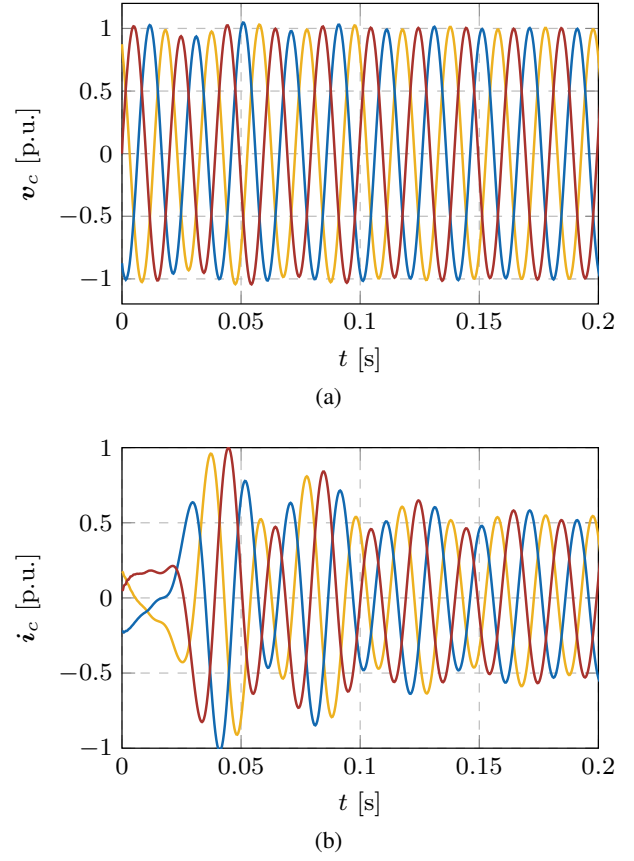
Fig. 5: Three-phase components at the converter output during start-up: (a) Instantaneous output voltages. (b) Instantaneous output currents.
