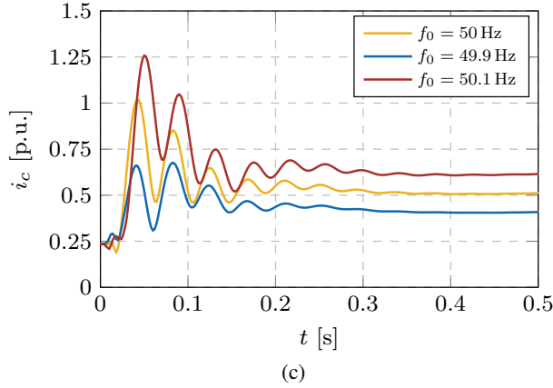
Fig. 6: Impact of initial rotor frequency term on the synchronization process of a VIM during start-up: (a) Frequency. (b) Output voltage. (c) Output current.
