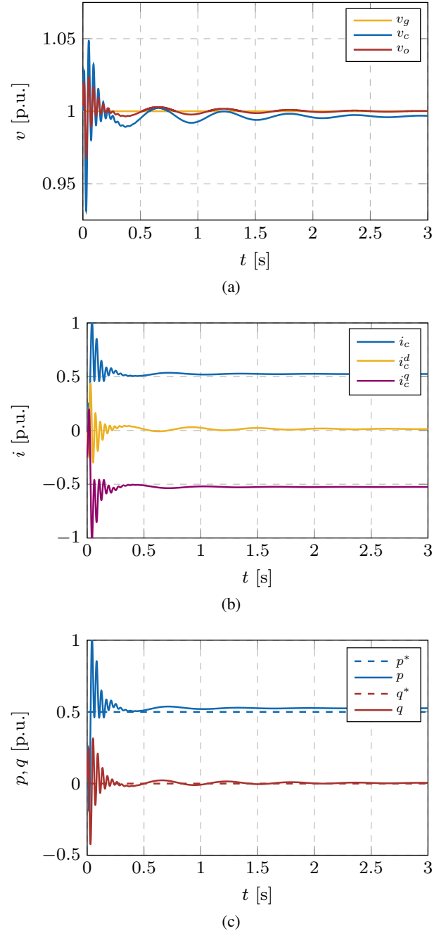
Fig. 3: Behavior of the converter emulated as a virtual induction machine during start-up: (a) RMS output voltages (before and after the filter). (b) RMS output current with dq -components. (c) Active and reactive power output and reference tracking.
